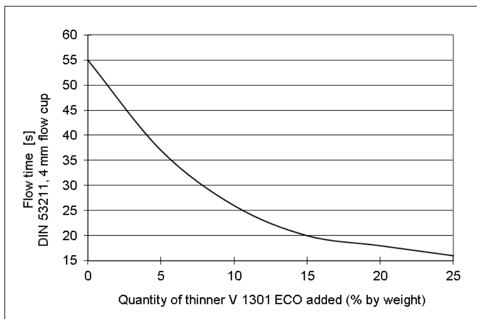
Fig. 1: Viscosity depending on the quantity of thinner added to conformal coating ELPEGUARD® SL 1301 ECO-FLZ at 20 °C [68 °F]
